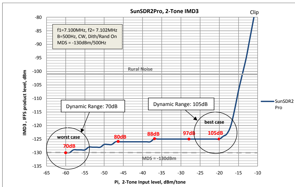
Fig. 1: IMD3-curve of a digital direct-sampling SDR
